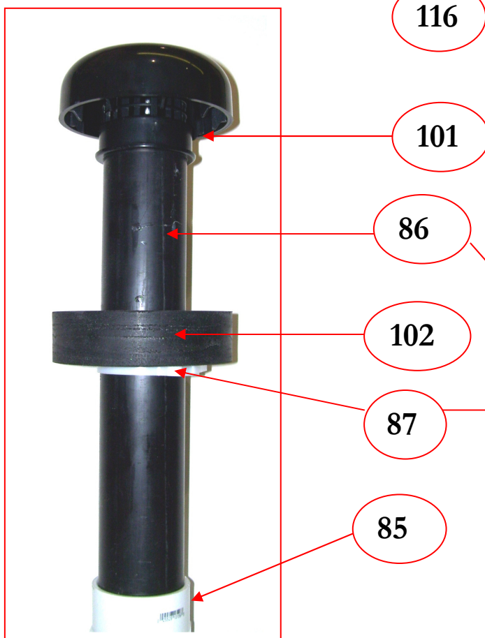
VACUUM SHUTOFF ASSEMBLY
